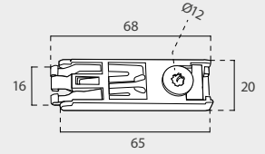
LOCK *mm
