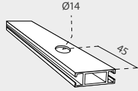
CONNECTOR *mm
